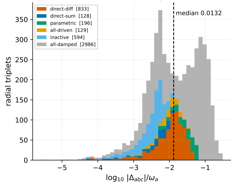
(a) 4866 radial triplets by channel
